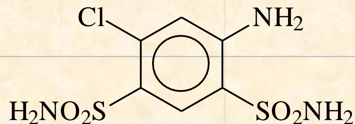
Chloraminophenamide
