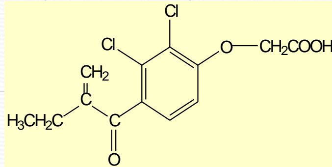
2,3-Dichloro-4-(2-methylene-1-oxobutyl)phenoxyacetic acid
