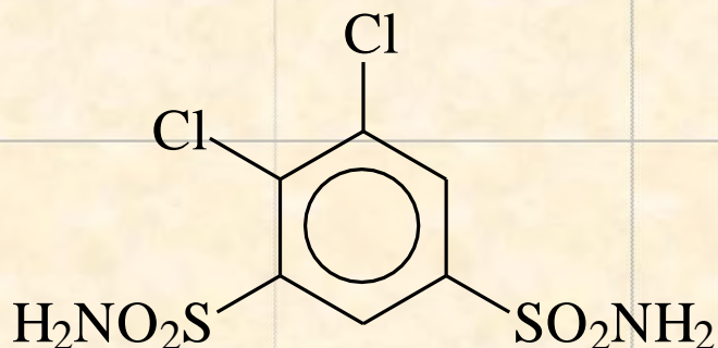
Dichlorphenamide ( Daramide )
