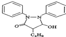
Phenylbutazone
