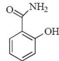
Salicylamide
