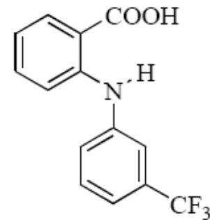
Flufenamic acid
