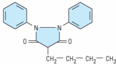
Phenylbutazone
