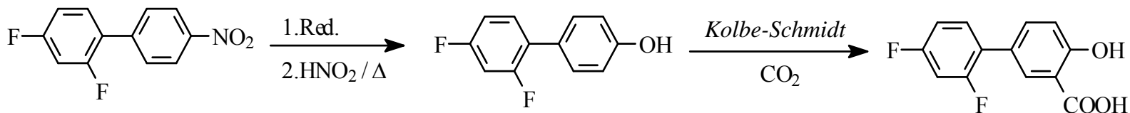
2',4'-difluoro-4-hydroxybiphenyl-3-carboxylic acid
