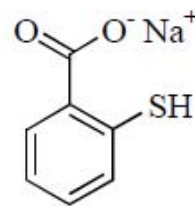
Sodium Thiosalicylate
